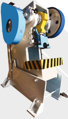
BSP Series, C Frame inclinable Power Press
